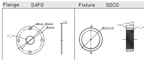
Unit: mm VRT10 Standard
