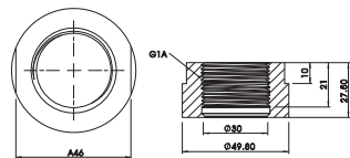
Unit: mm
